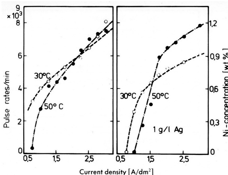
Figure 26 - Nickel content of gold-nickel deposits from an alkaline cyanide bath (10 g/L Au, 3 g/L Ni doped with 63 Ni, 150 g/L KCN).
