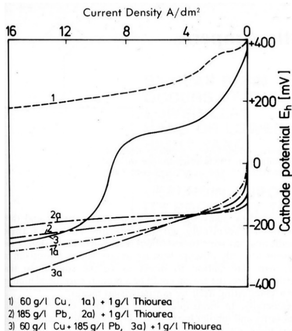
Figure 16 - Cathode potential-current density curves of copper and lead in acid perchlorate solutions with and without thiourea, at 25°C and quiescent electrolyte.
