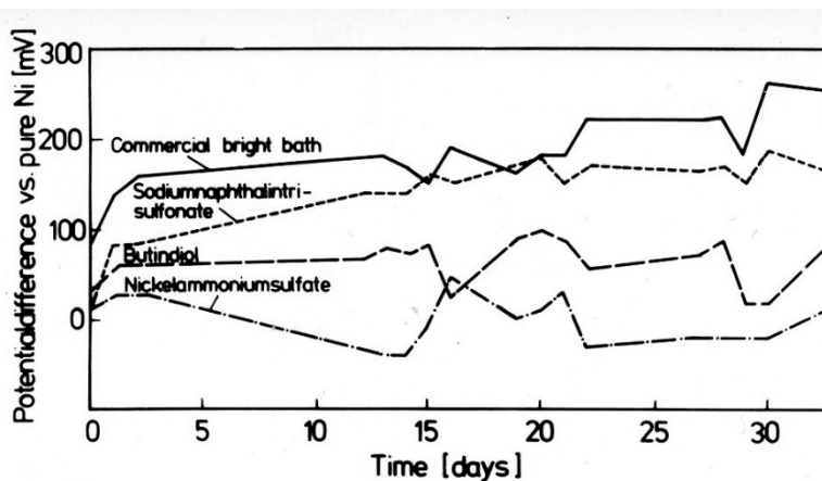
Figure 9 - Potential difference between pure electrolytic nickel and nickel from baths with different addition agents in 3% sodium chloride solution with a pH of 3 at room temperature.
