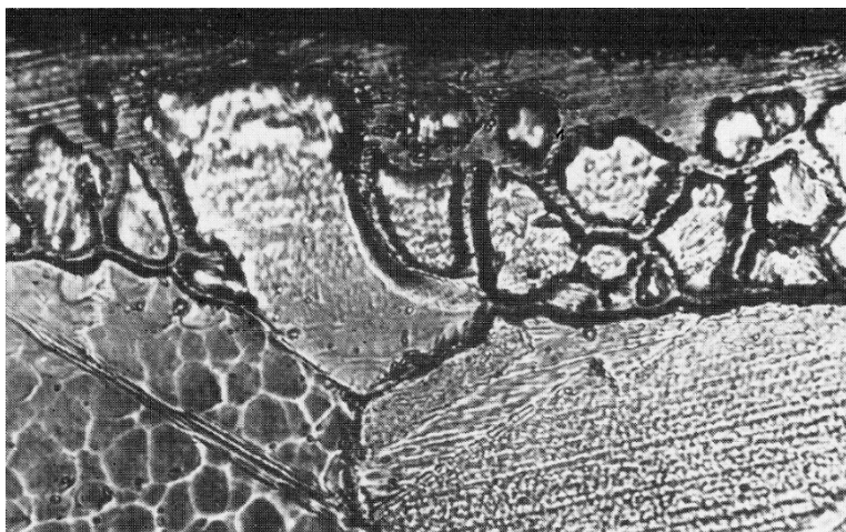
Figure 46 - Diffusion of gold and silver in gold-plated silver during annealing.
