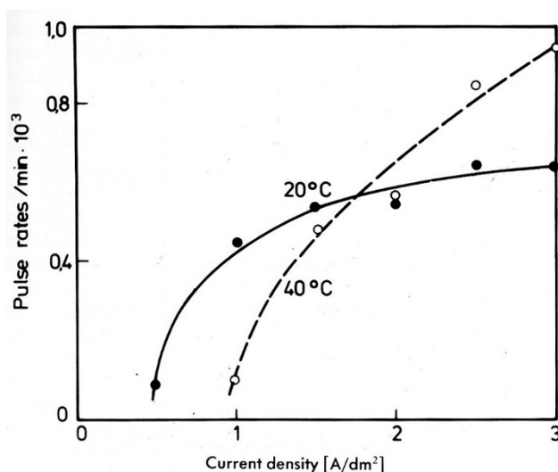
Figure 18 - Impulse rates of silver deposits from a cyanide electrolyte with 5 g/L Ag and 30 g/L Ni doped with ^{63}\text{Ni} .
