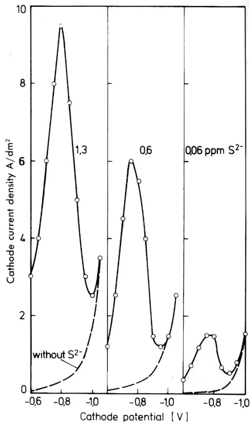
Figure 10 - Potentiostatic potential-current density curves in a cyanide silver electrolyte with and without additions of S^{2-} ions. Electrolyte composition 200 g/L KCN and 80 g/L Ag as KAg(CN)_2 .
