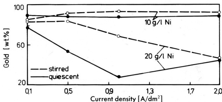
Figure 27 - Gold content of gold-nickel deposits from a citric acid bath with 2 g/L Au as KAu(CN) 2 , 10 or 20 g/L Ni as NiSO 4 , 60 g/L sodium citrate and 40 g/L citric acid; pH 4.2; 40°C.
