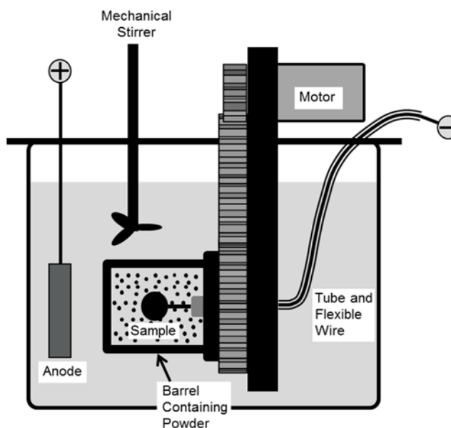
Figure 1 - Schematic of the barrel system.
