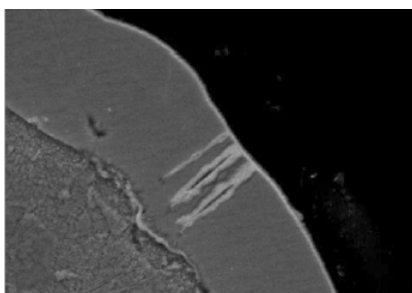
(b) Phos-Pd = 4.8 \mu -in. (0.12 \mu m)
