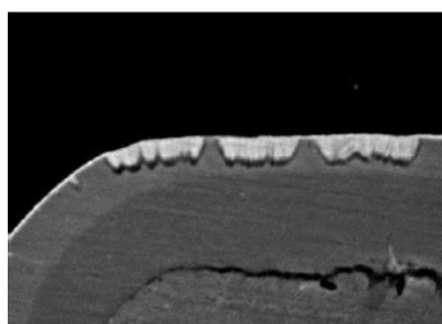
(a) Phos-Pd = 2.0 \mu -in. (0.05 \mu m)
