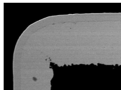
(c) Phos-Pd = 8.8 \mu -in. (0.22 \mu m)
