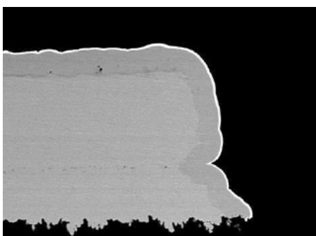
(b) Phos Pd = 6.4 \mu -in. (0.19 \mu m)
