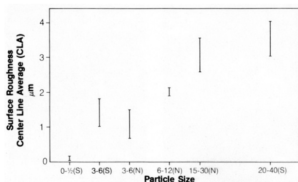
Figure 10 - Surface roughness of nickel electrodeposits containing (S) synthetic and (N) natural diamond particles.
