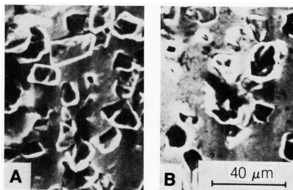
Figure 3 - SEM surface micrographs of deposits formed on vertical cathode in nickel sulfamate bath (at 50°C) containing 50 carat/L of 20- to 40- \mu\text{m} synthetic diamonds at (a) 1 A/dm 2 and (b) 3 A/dm 2 . Agitation was intermediate ( n = 0 ).
