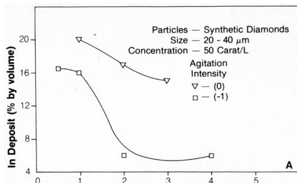
Figure 1 - Concentration of synthetic diamonds in nickel deposits as a function of current density.
