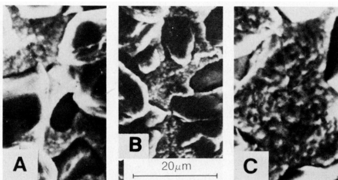
Figure 6 - SEM surface views of deposits produced at 4 A/dm 2 in nickel sulfamate solution (at 50°C) containing 125 carat/L of 15- to 30- \mu\text{m} natural diamonds using: (a) a horizontal cathode and magnetic stirrer at 180 rpm, (b) a horizontal cathode and magnetic stirrer at 360 rpm, and (c) a vertical cathode and magnetic stirrer at 180 rpm.
