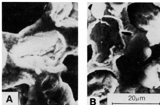
Figure 13 - SEM micrographs showing voids in nickel deposits created by the dislodgement of 20- to 40-μm synthetic diamond particles: (a) deposit at 1 A/dm 2 on a vertical cathode and (b) deposit at 1 A/dm 2 on a horizontal surface.
