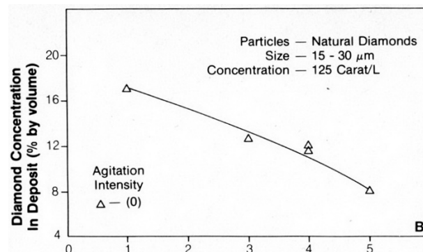
Figure 2 - Concentration of natural diamond particles in nickel deposits as a function of current density.
