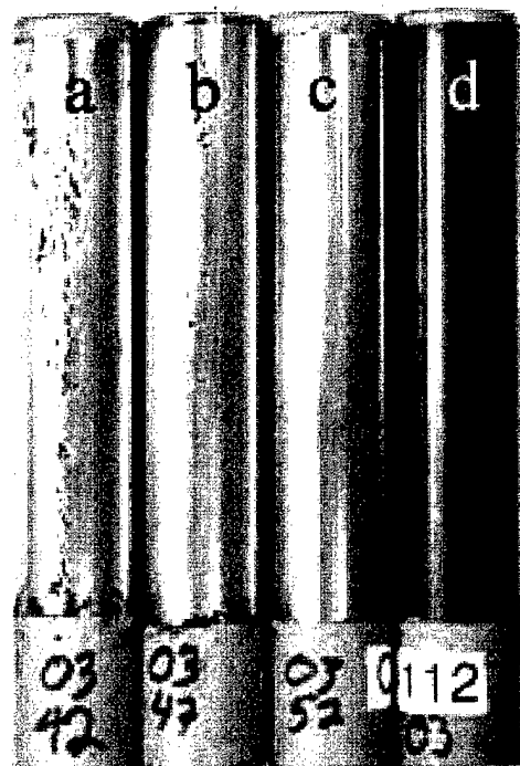
Figure 3-39. Coatings on 4340 Steel After the B117 Test: a) EHC Coating Only b) EHC with Sealer, c) EHC with Ni Sublayer, and d) 0.010\"
