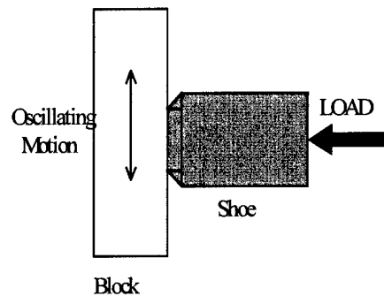
Figure 3-66 Cross-sectional Schematic of Fretting Wear Test
