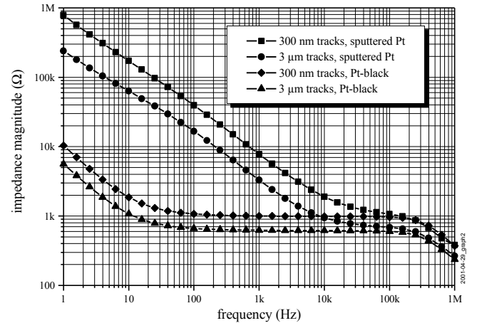
Fig. 3: Spectra of impedance magnitudes of dot-shaped electrodes ( \varnothing=500 \mu\text{m} , connected to integrated interconnection lines), made of different material combinations: sputtered platinum on sputtered tracks (square), sputtered platinum on electroplated tracks (dot), platinum black on sputtered tracks (diamond), and platinum black on electroplated tracks (triangle). Measured in 0.9% NaCl solution, 100 mV sine excitation at room temperature.
