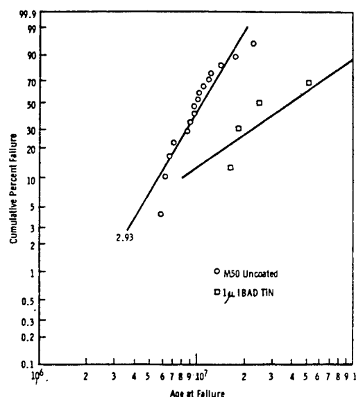
FIG. 7 Weibull distribution of RCF tests comparing M50 alloy uncoated rod vs. IBAID treated rod. Results demonstrate significantly extended lifetime for IBAID TiN at 50% lifetime (B50 lifetime). From [33].
