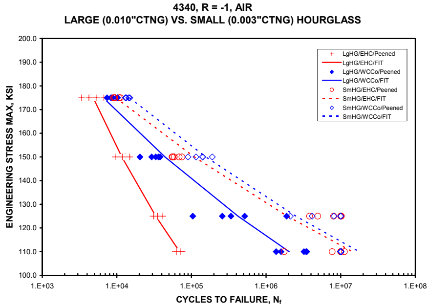
Figure 10. Fatigue Data for EHC Compared to HVOF WC/17Co in Air on Hourglass Specimens at R = -1.
