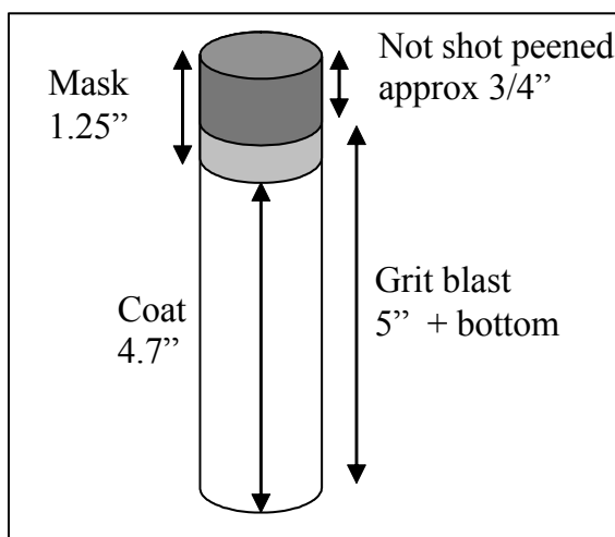
Figure 6. Schematic of Corrosion Specimen.
