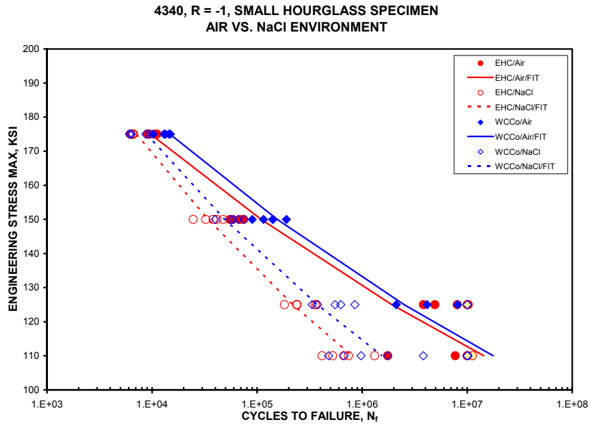
Figure 11. Fatigue Data for EHC Compared to HVOF WC/17Co for .003" Thickness at R = -1 in Air or NaCl Solution.
