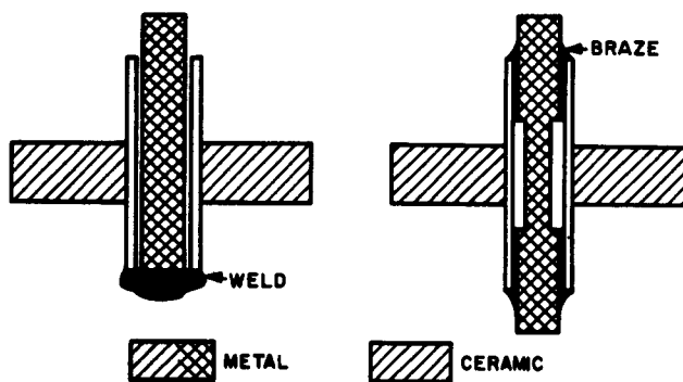
FIGURE 5. HOLLOW-PIN SEALS STRENGTHENED WITH SOLID PIN INSERT
