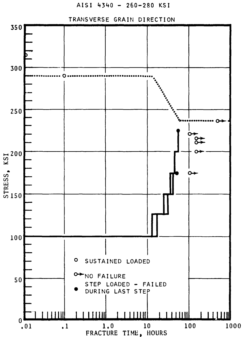
FIGURE 5 - SUSTAINED LOAD - .003 NOTCH - PLATED BY BENDIX - SOUTH BEND (DALIC BRUSH) TESTED BY CONVAIR-FORT WORTH
