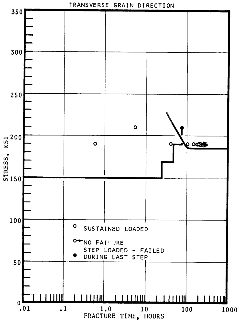
FIGURE 8 - SUSTAINED LOAD - .003 NOTCH - PLATED BY BOEING-RENTON (CADMIUM-TITANIUM BAC 5804) TESTED BY MARTIN-BALTIMORE
