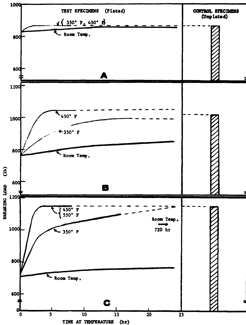
Figure 8. The Effect of Relief Treatments on Breaking Load of Cyanide Cadmium Plated Half-ring Specimens (4340 steel) at A - 180,000 psi Ultimate Tensile Strength B - 230,000 psi Ultimate Tensile Strength C - 270,000 psi Ultimate Tensile Strength
