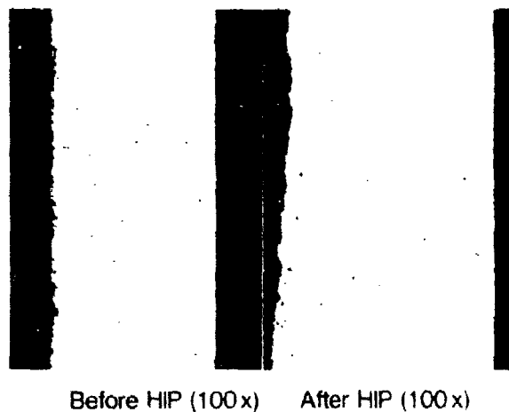
Figure 9 Microsections of blades before and after HIP treatment
