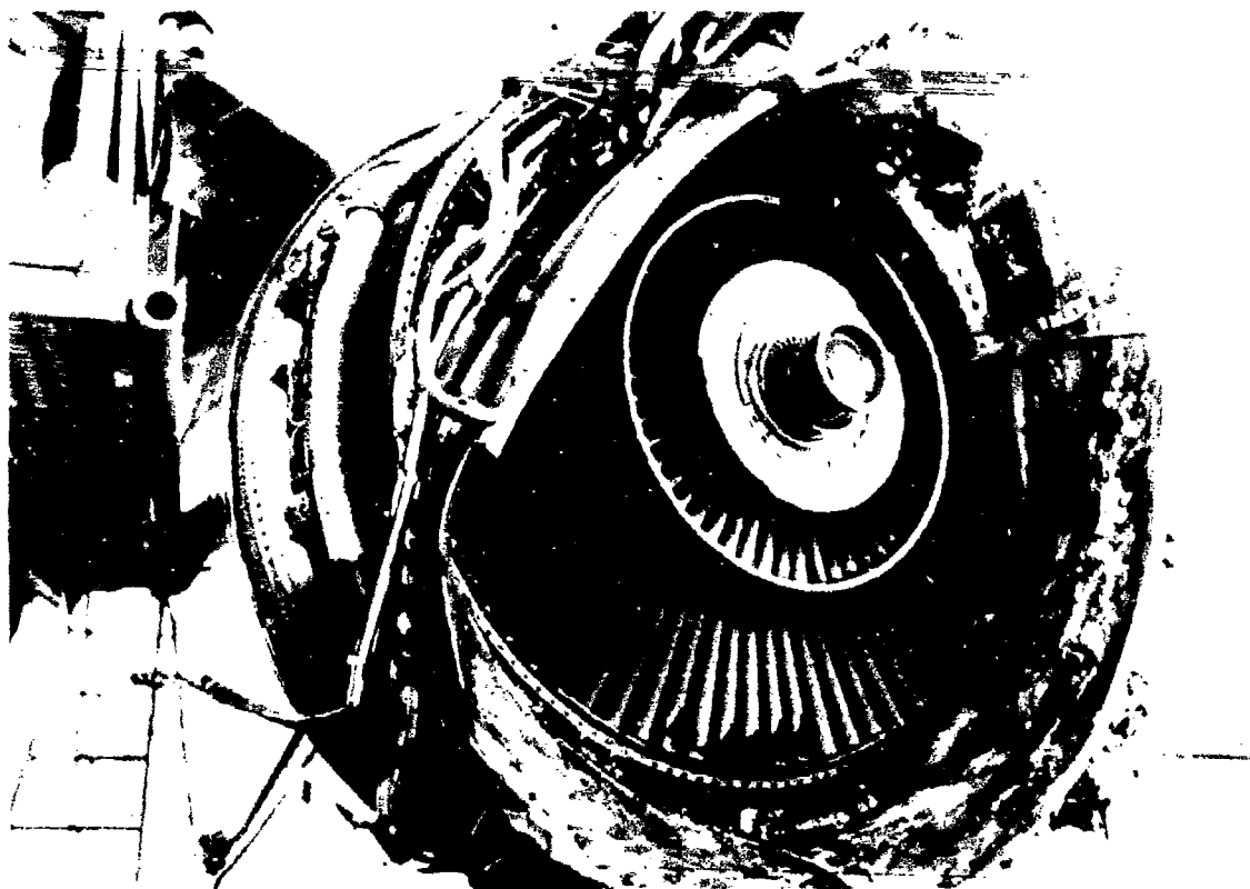
Fig.7 - Effects of a Fan Disc Failure
