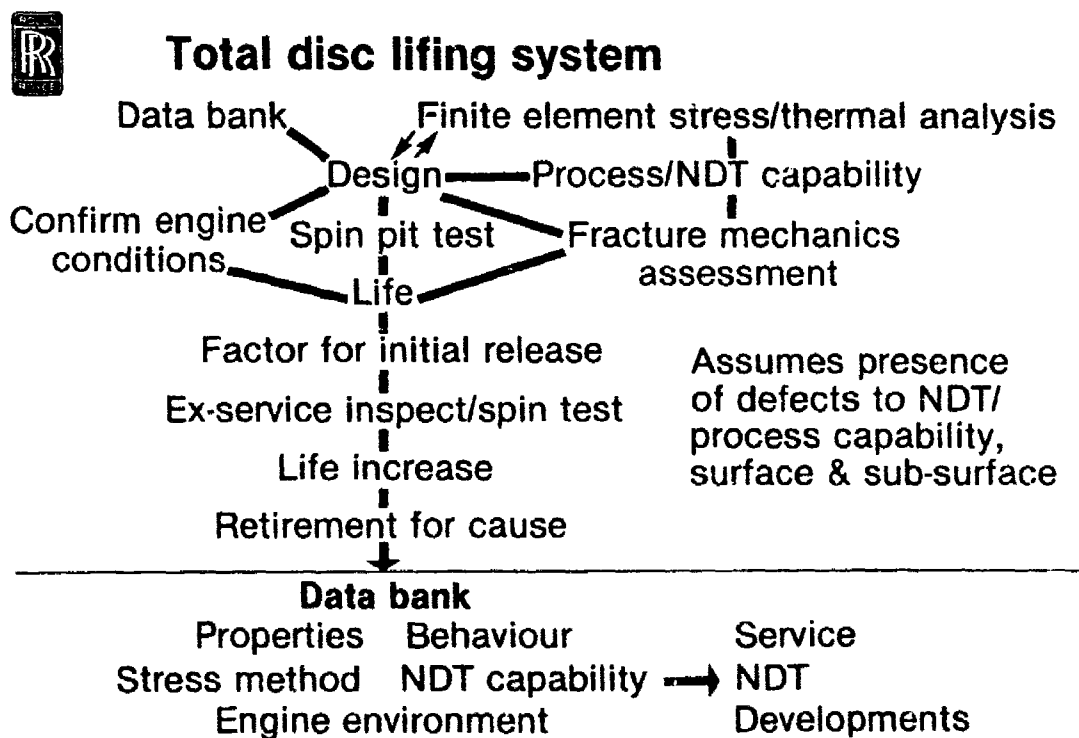
Fig.14 - Total Disc Lifing System
