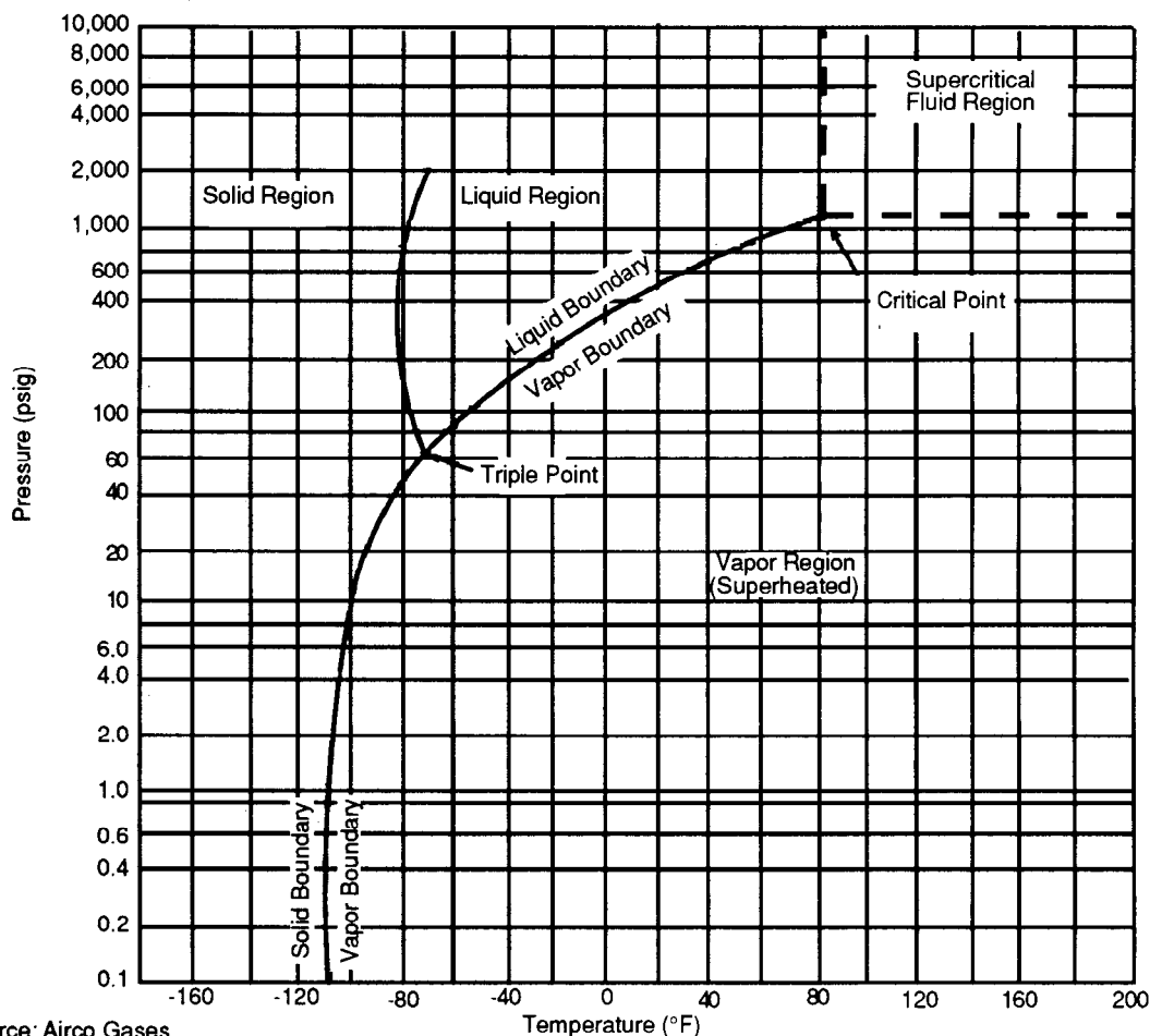
Figure 1. Phase diagram for pure \text{CO}_2 .
