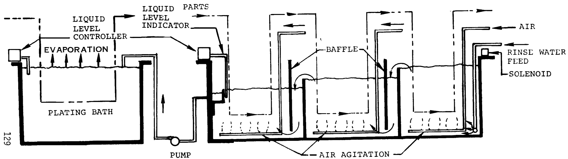
FIGURE 7-6 CLOSED LOOP 3 STAGE COUNTER CURRENT RINSE
