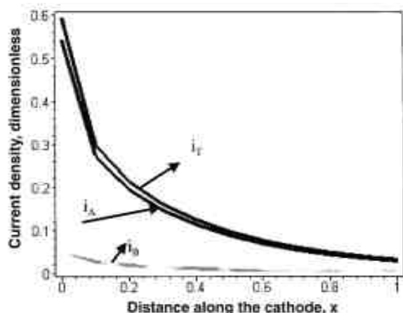
Fig. 4—Predicted partial current densities in an Hull cell.
