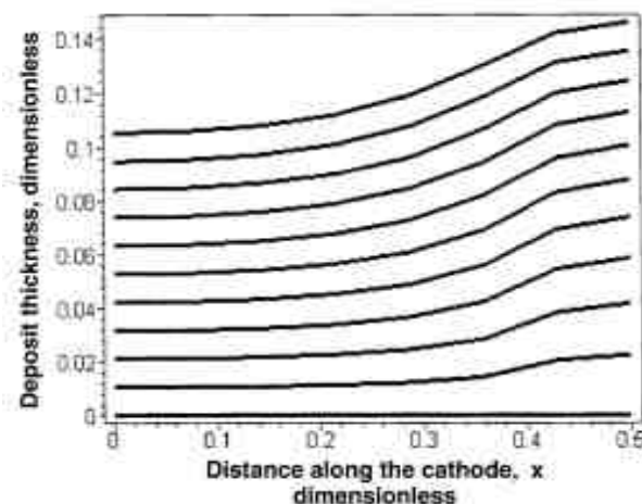
Fig. 6—Growing metal deposit predicted by semianalytical method.
