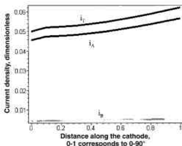
Fig. 5—Predicted partial current densities along the cylindrical bearing anode.
