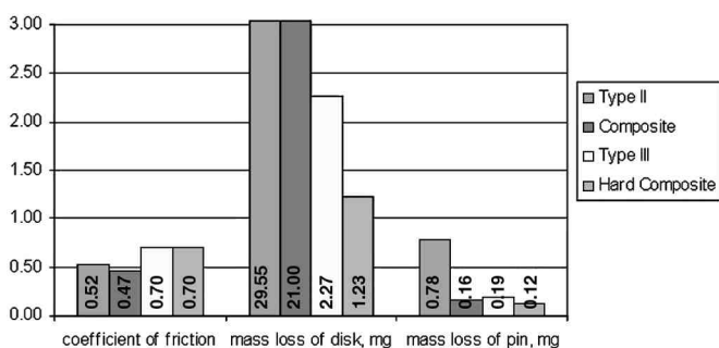
Fig. 5—Pin-on-Disk test results. Note the range in mass loss values for the finished disk samples and correspondence to the Taber abrasion data, especially for the mass loss of the pin.
