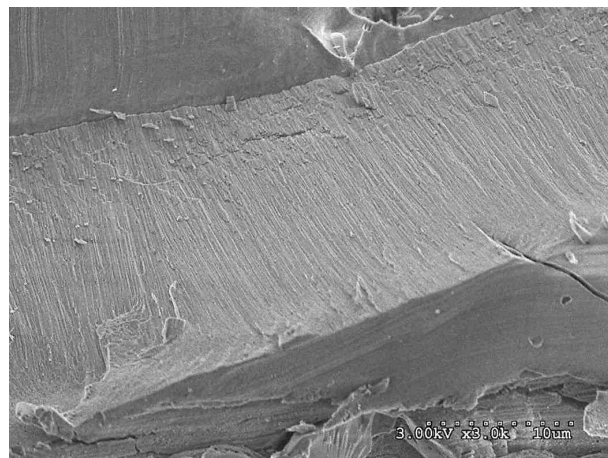
Fig. 4—Ductile fracture surface of the hard version of the composite-finished Charpy impact sample.
