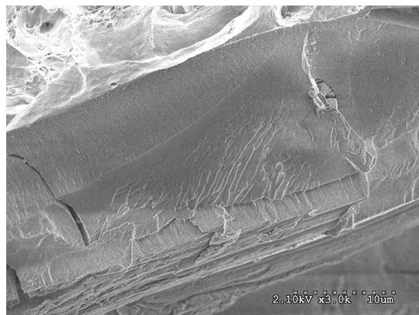
Fig. 3—Brittle fracture surface of Type III-finished Charpy impact sample.
