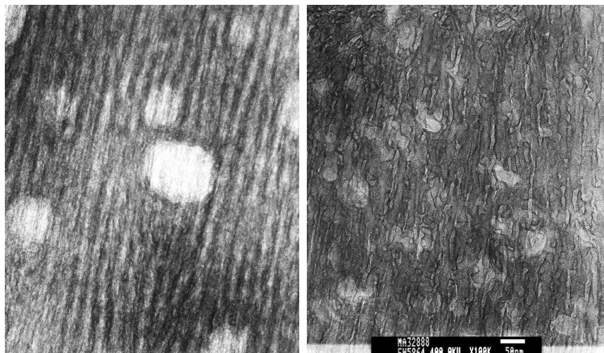
Fig. 7—Type II microstructure (left); composite microstructure (right). Note how the unidirectional columns of the Type II structure (left) have become more skewed and random—with the change in electrolyte yielding the composite structure on the right.
