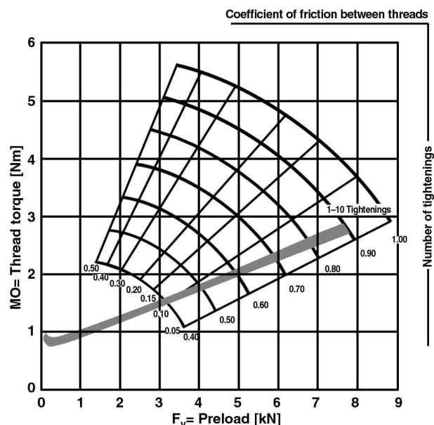
Fig. 6—Torque test data for composite finished aluminum fastener, \text{MoS}_2 lubricant and steel bolt. The data band represents all 10 load excursions. The data overlap indicates the finish exhibits good antigalling properties.
