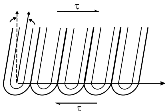
Fig. 1—Schematic of the columnar structure of the anodic finish under applied shear force ( \tau ). The angle represents displacement of the structure through elastic deformation.
