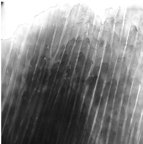
Fig. 8—Top surface of Type III finish after exposure to shear forces. Note the structure has chipped off across the tops of the columns.
