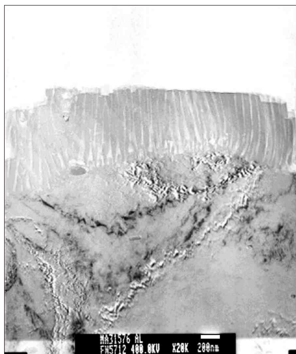
Fig. 2—Crystallographic defects impact the way the anodic oxide finish nucleates and grows.
