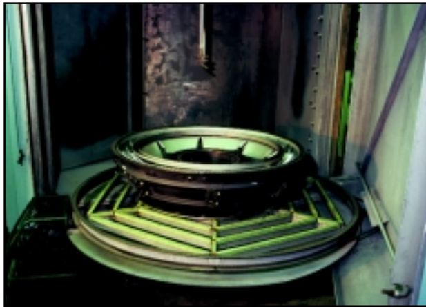
Large jet engine mid-frame case and the center nozzle lance.
