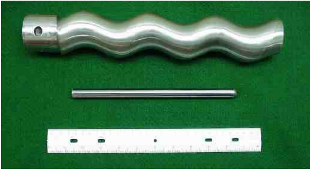
Figure 5: Parts to be chromium plated
