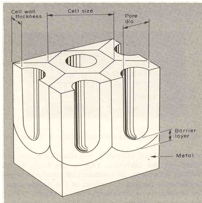
Figure A. Microstructure of Anodic Film
