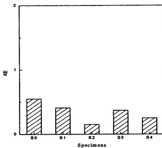
Figure 3 - Anti-finger property with silica content.
