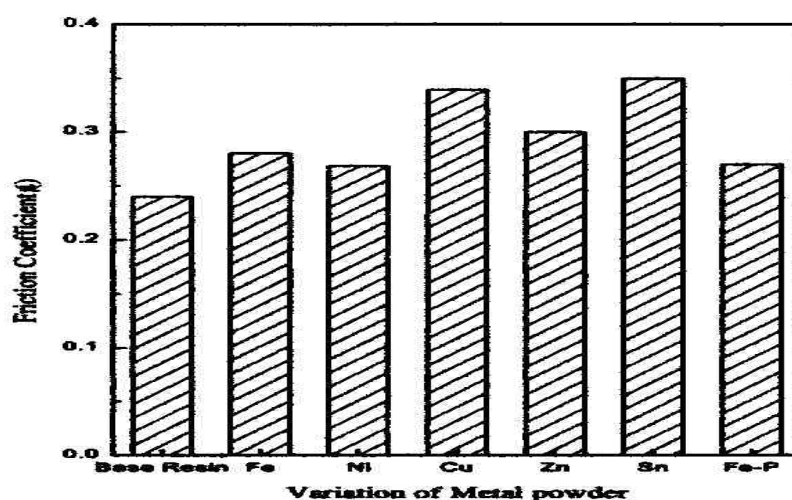
Figure 11 - Comparison of friction coefficient
