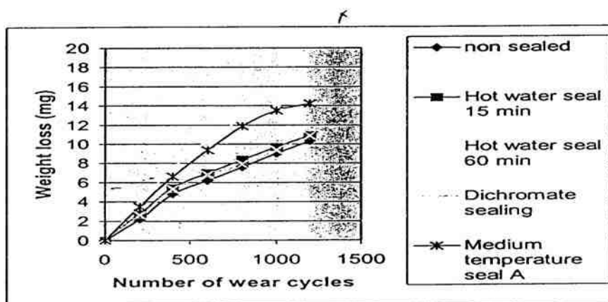
Figure 10 - Abrasive wear resistance hard anodic coatings with conventional sealing methods.
