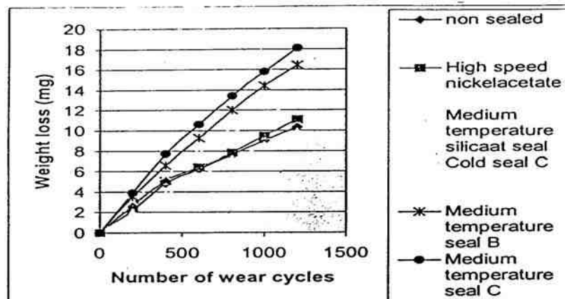
Figure. 9 - Abrasive wear resistance hard anodic coatings with different sealing methods.
