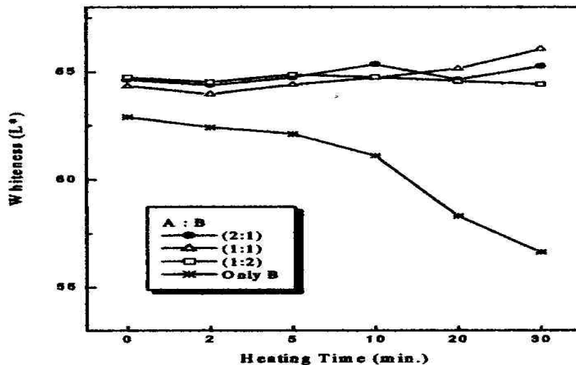
Fig 5 – Changes of whiteness for various resins
