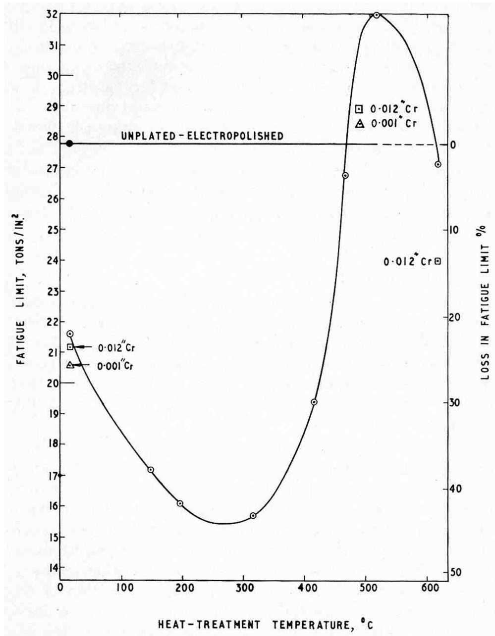
Figure 7 - Effect of baking on fatigue limit; En 25 steel DPH 305; 6 mil chromium. 6
