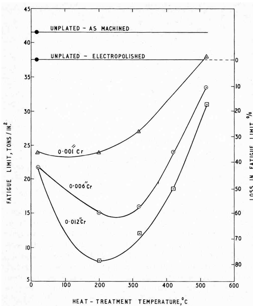
Figure 6 - Effect of baking on fatigue limit for three thicknesses of chromium; En 25 steel, DPH 400. 6
