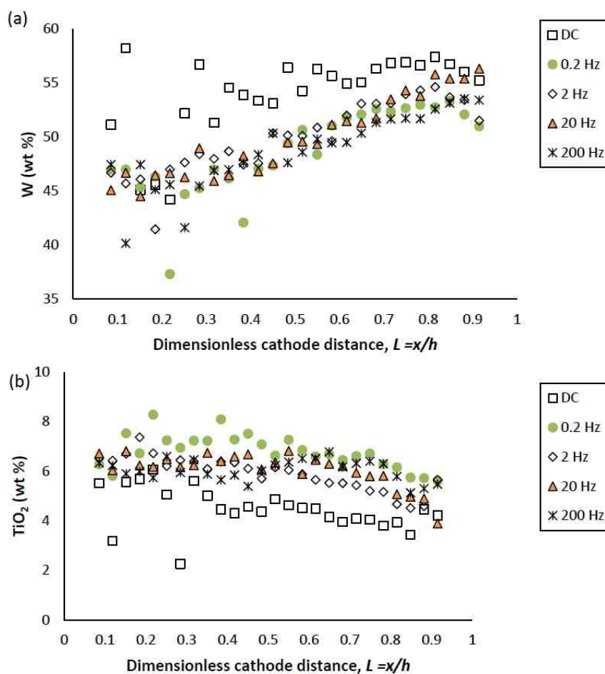
Figure 1 - Ni-W-TiO 2 deposit composition of (a) tungsten and (b) TiO 2 (wt%) under DC and PC (with variable pulse frequency) conditions, with respect to a dimensionless length L representing lower and higher current densities with smaller and larger values, respectively.
