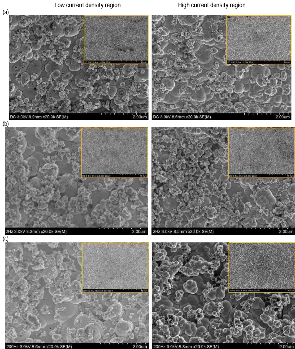
Figure 3 - SEM images of Ni-W-TiO 2 deposits plated with (a) DC, (b) PC with the frequency of 2 Hz and (c) PC with the frequency of 200 Hz, in low current density (left) and high current density (right) regions, at low (5K, inset, upper right) and high (20K) magnifications.
