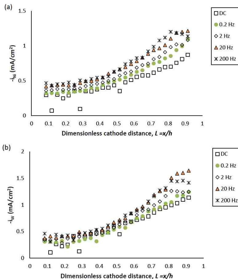
Figure 2 - Partial current density of (a) nickel and (b) tungsten under DC and PC (with variable pulse frequency) condition, with respect to a dimensionless length L representing lower and higher current densities with smaller and larger values, respectively.
